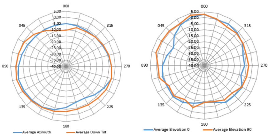
Azimuth plane (top view)
